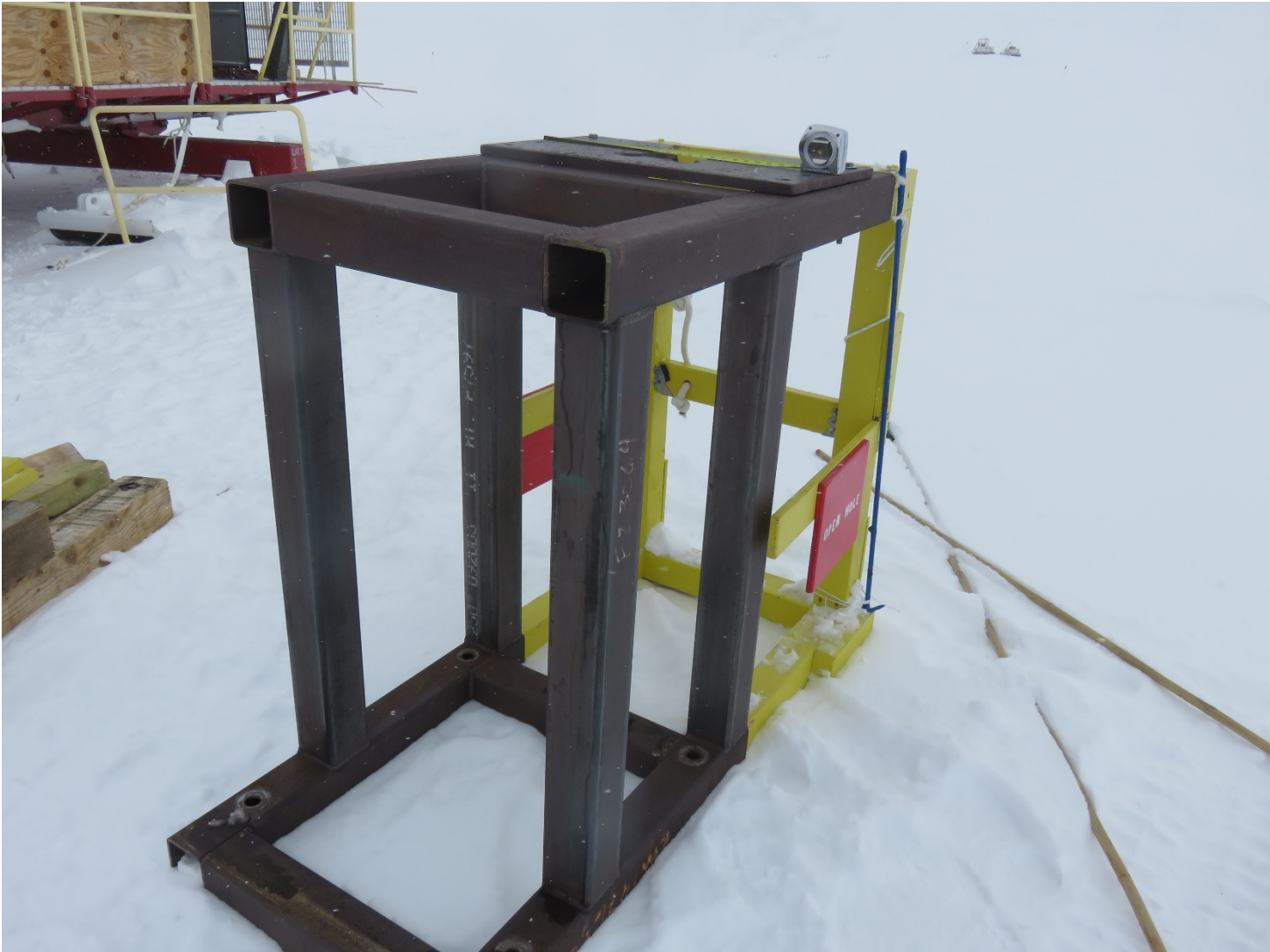
Tool assembly frame after removal from LARS deck.
